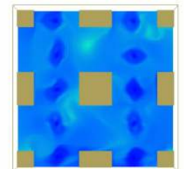
CFD modelling to demonstrate air change effectiveness
